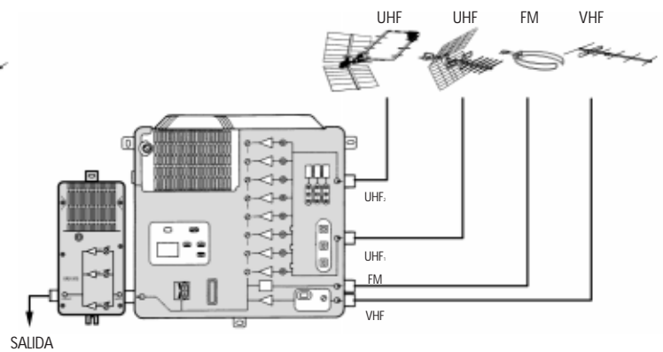
MICROMATV + SAB 252
