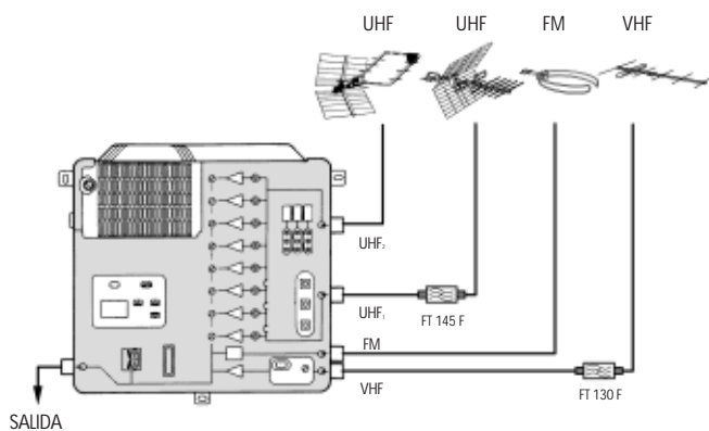
MICROMATV
