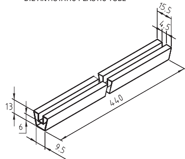
DIL ANTISTATIC PLASTIC TUBE
